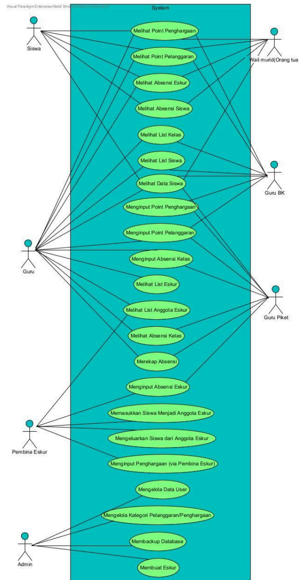
Gambar 3.2.1 Use case Diagram
